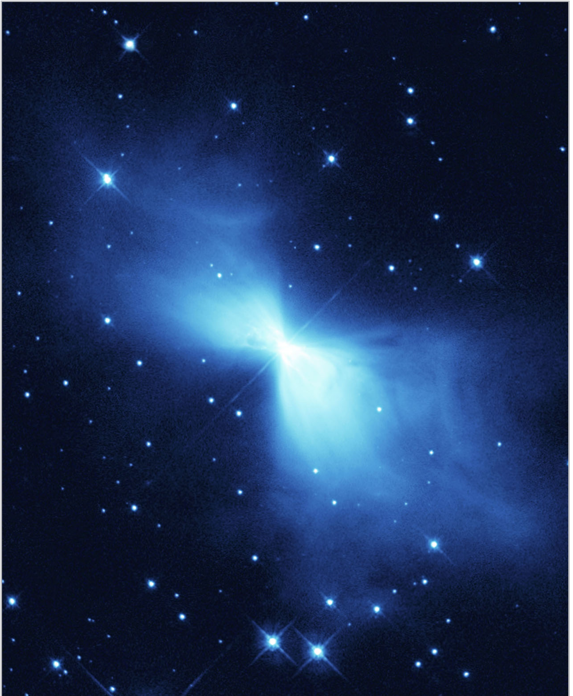
The Boomerang Nebula is a young planetary nebula and the coldest object found in the Universe so far. The NASA/ESA Hubble Space Telescope image is yet another example of how Hubble's sharp eye reveals surprising details in celestial objects.
