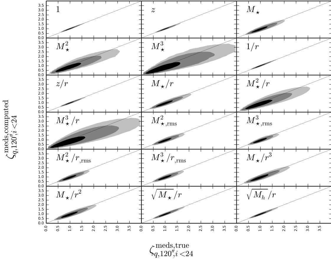
Figure 9. Same as Figure 8, but for \zeta_q^{i \in \text{MS,meds}} .
