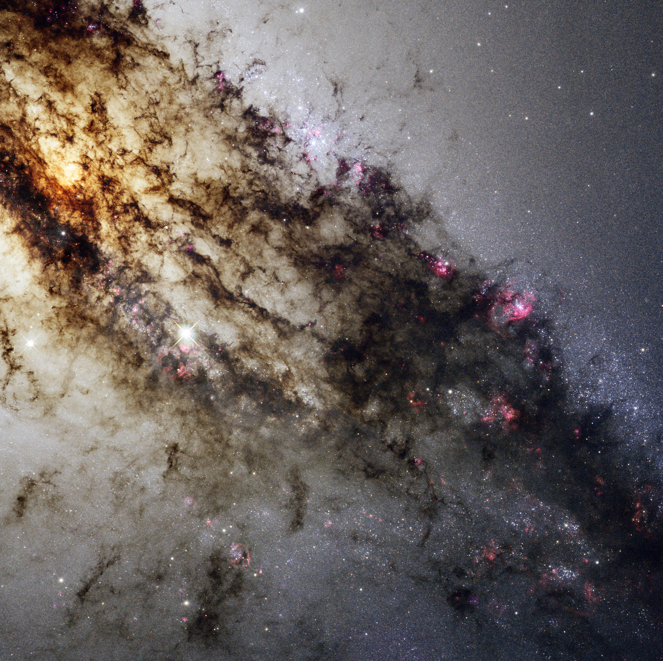
A spectacular view of Centaurus A
